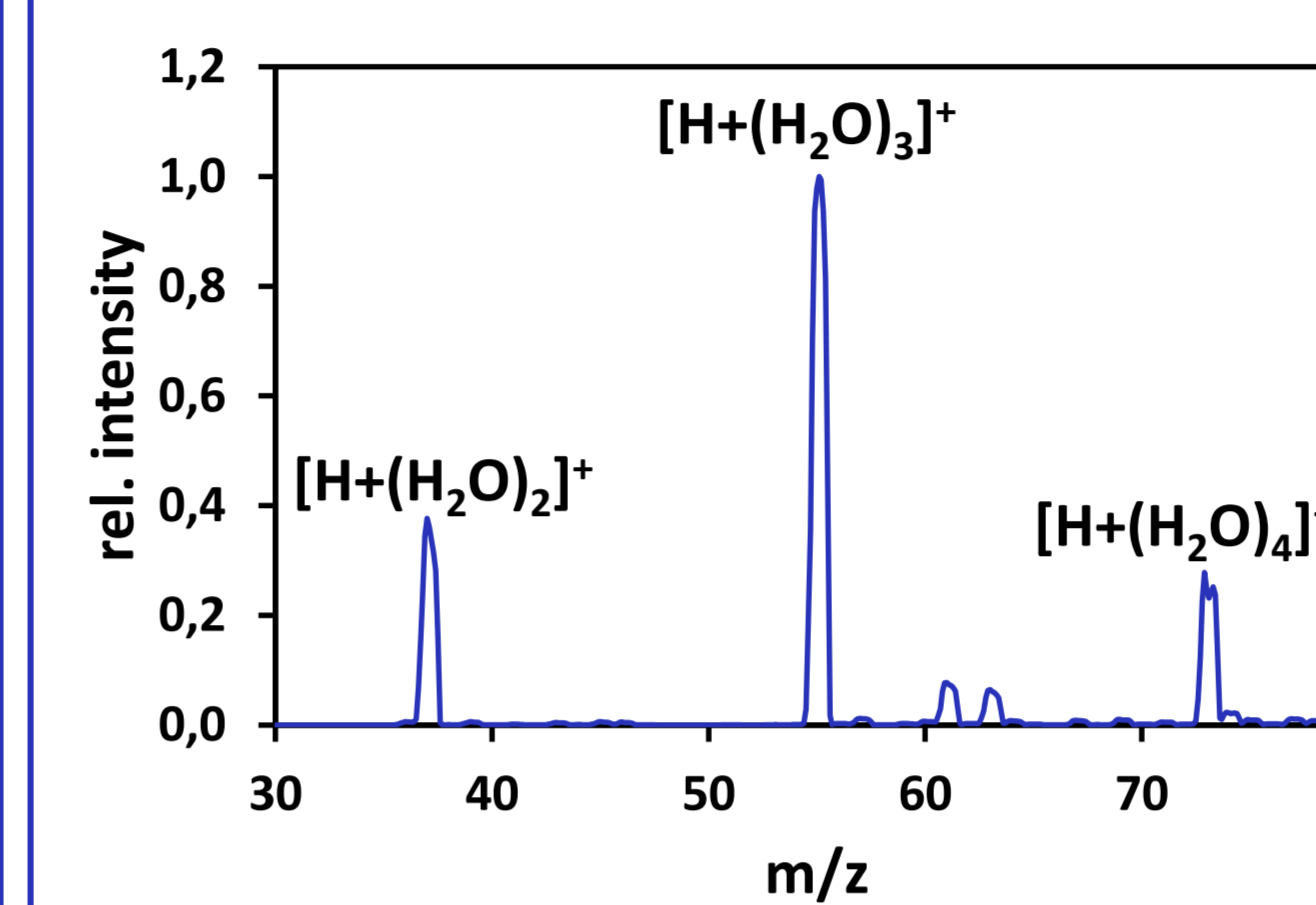
Figure 4: Water cluster distribution (6500 Triple Quad (Sciex))
